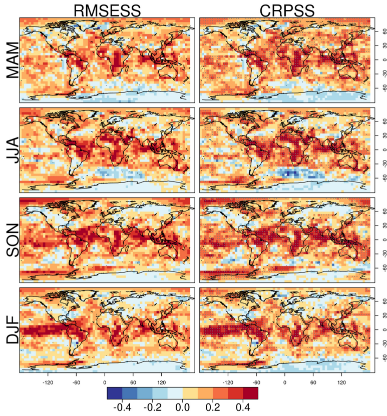
Figure 5. As Fig. 3 but for PREC.
