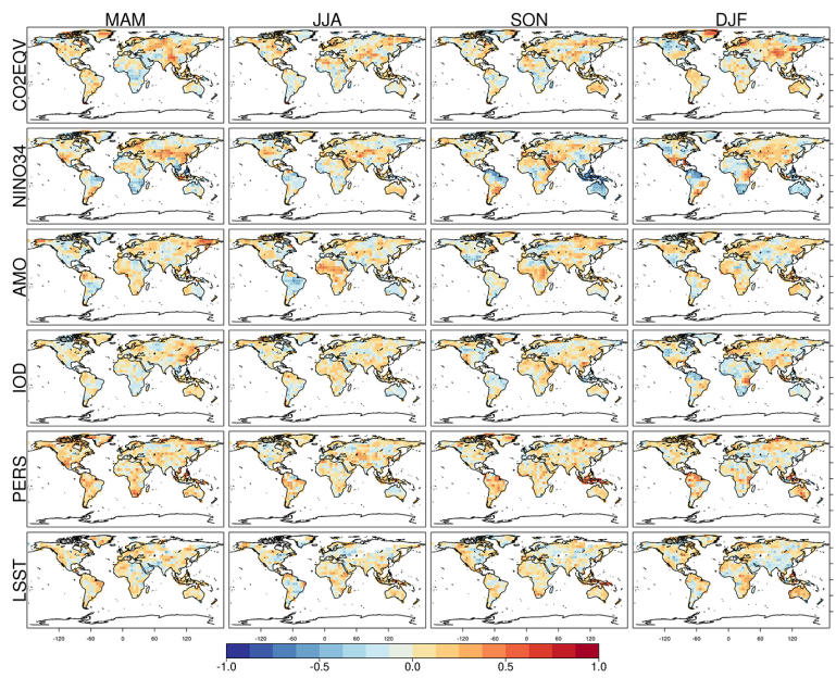
Figure 2. Correlation between seasonal PREC and the set of predictors with a one month lead time. As in Fig. 1, correlation between CO2EQV is shown in the top line; subsequent lines show correlation between predictand-predictor pairs following removal of the CO2EQV trend.
