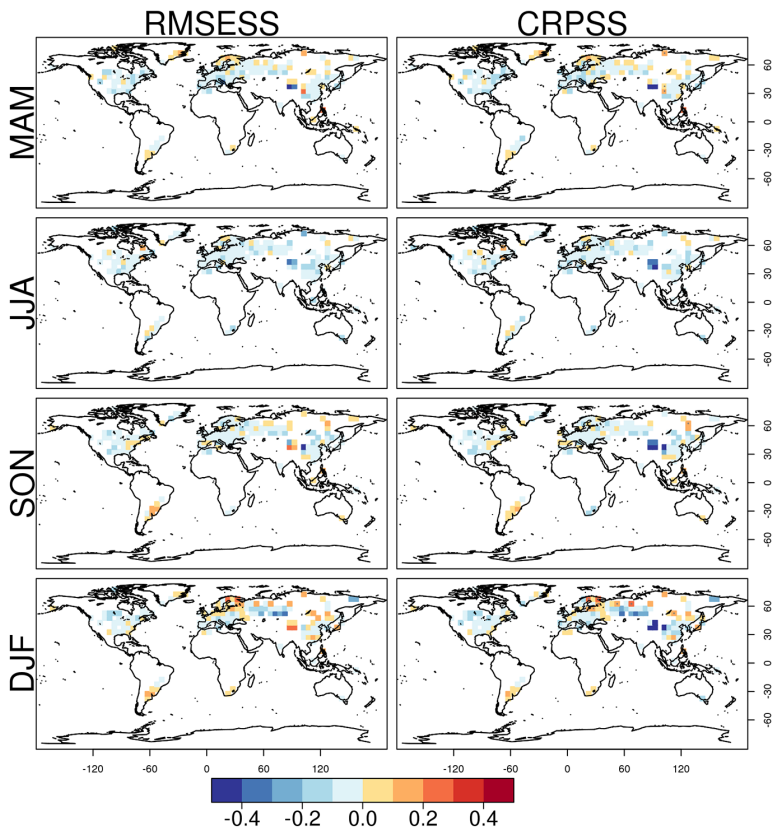
Figure 6. As Fig. 4 but for PREC.
